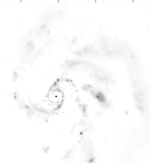
Residual
